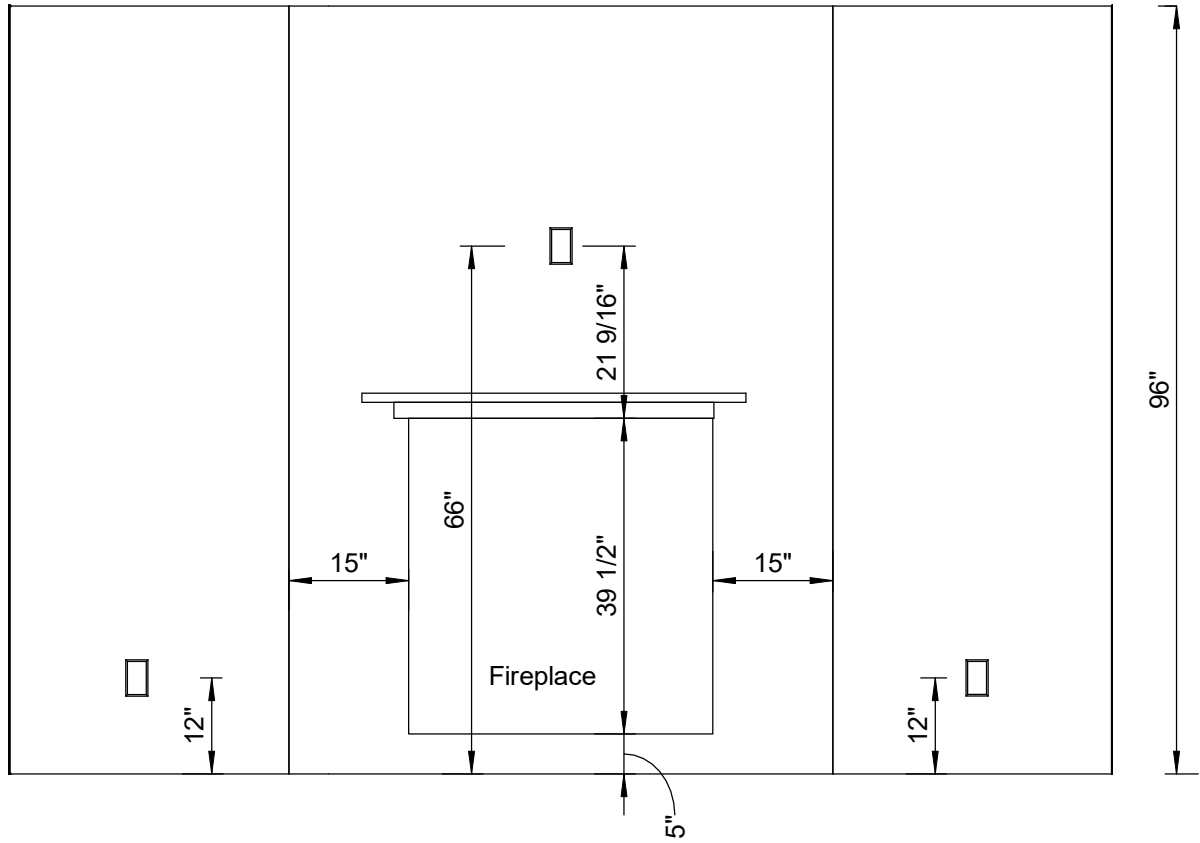
2 View 1 1/2" = 1'-0"
